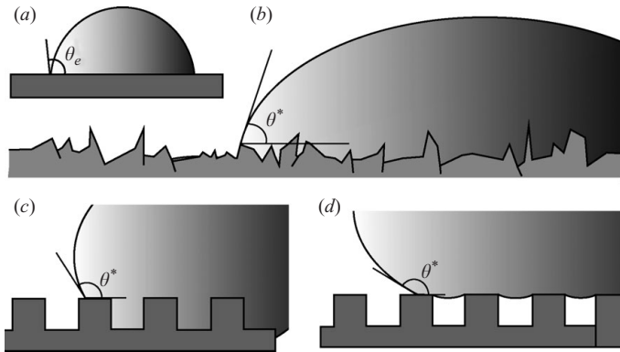
FIGURE 9. Roughening a surface will amplify its wetting tendencies: ( a ) \theta_e defines the equilibrium or chemical contact angle on a flat surface. ( b ) On a rough surface, the microscopic contact angle remains \theta_e , but the observed contact angle on the macroscopic scale, \theta^* , depends explicitly on the surface roughness. The two generic states of wetting, the Wenzel and Cassie states, are shown schematically in ( c ) and ( d ). In the Wenzel state, the pores are impregnated by fluid, increasing the fluid–solid contact. In the Cassie state, air pockets are trapped by the overlying fluid, reducing the fluid–solid contact.
